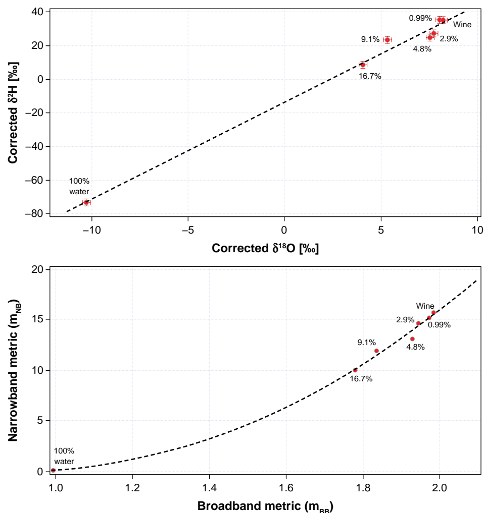
Figure 4 Identifying watering of a wine sample.
